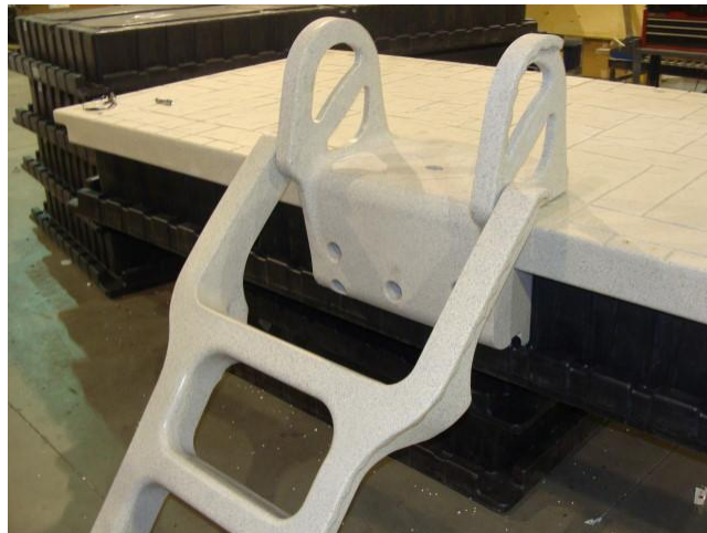
Completed Installation
